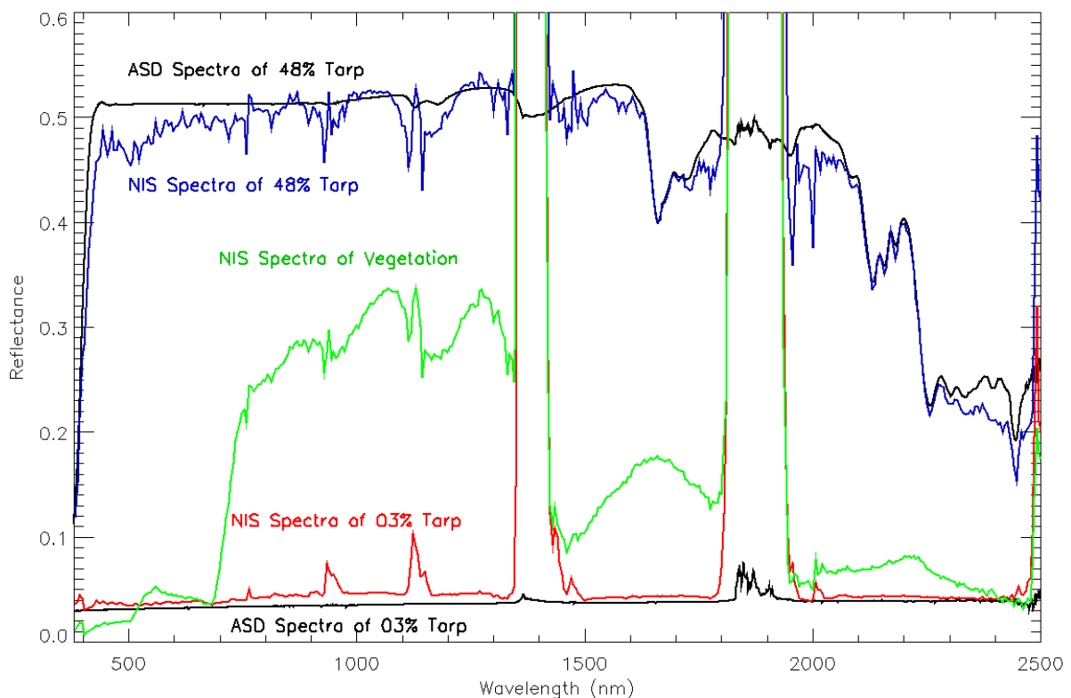
Figure 42: The as-delivered reflectance of calibration tarps (03% tarp in red and the 48% tarp in blue) and a vegetation pixel (green) measured by the airborne NEON Imaging Spectrometer. Noise and atmospheric artifacts are seen in the NIS curves. The black curves are ground truth reflectance measured by an ASD spectrometer
