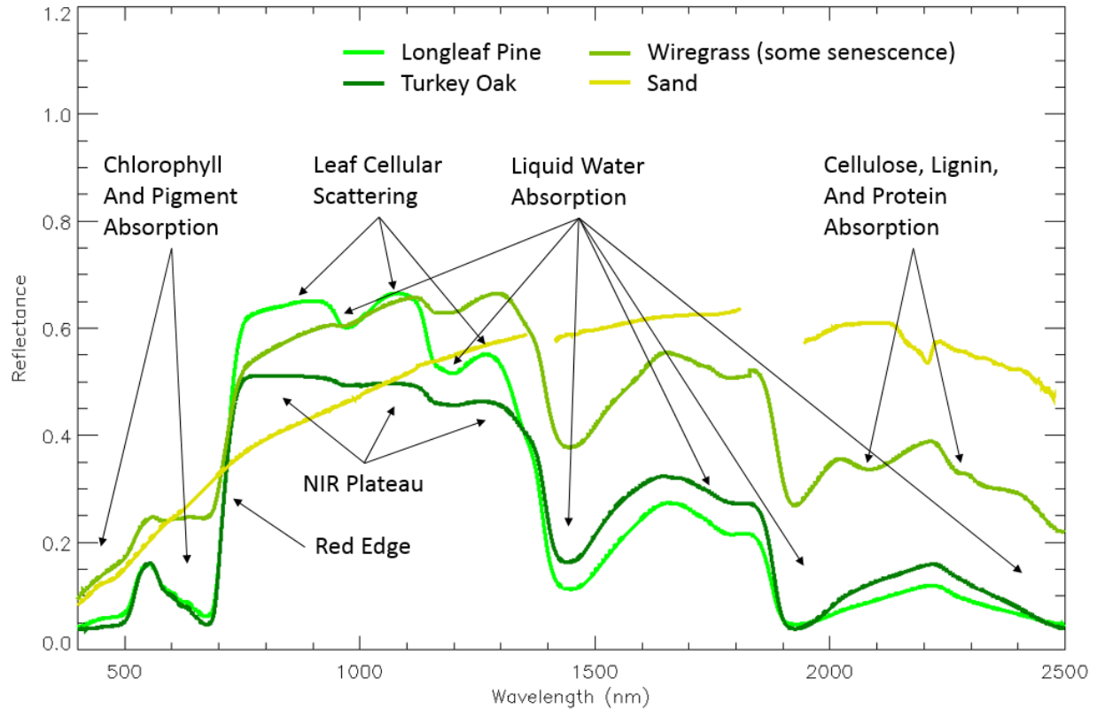
Figure 1: Reflectance curves of ground targets showing absorption and scattering spectral traits
