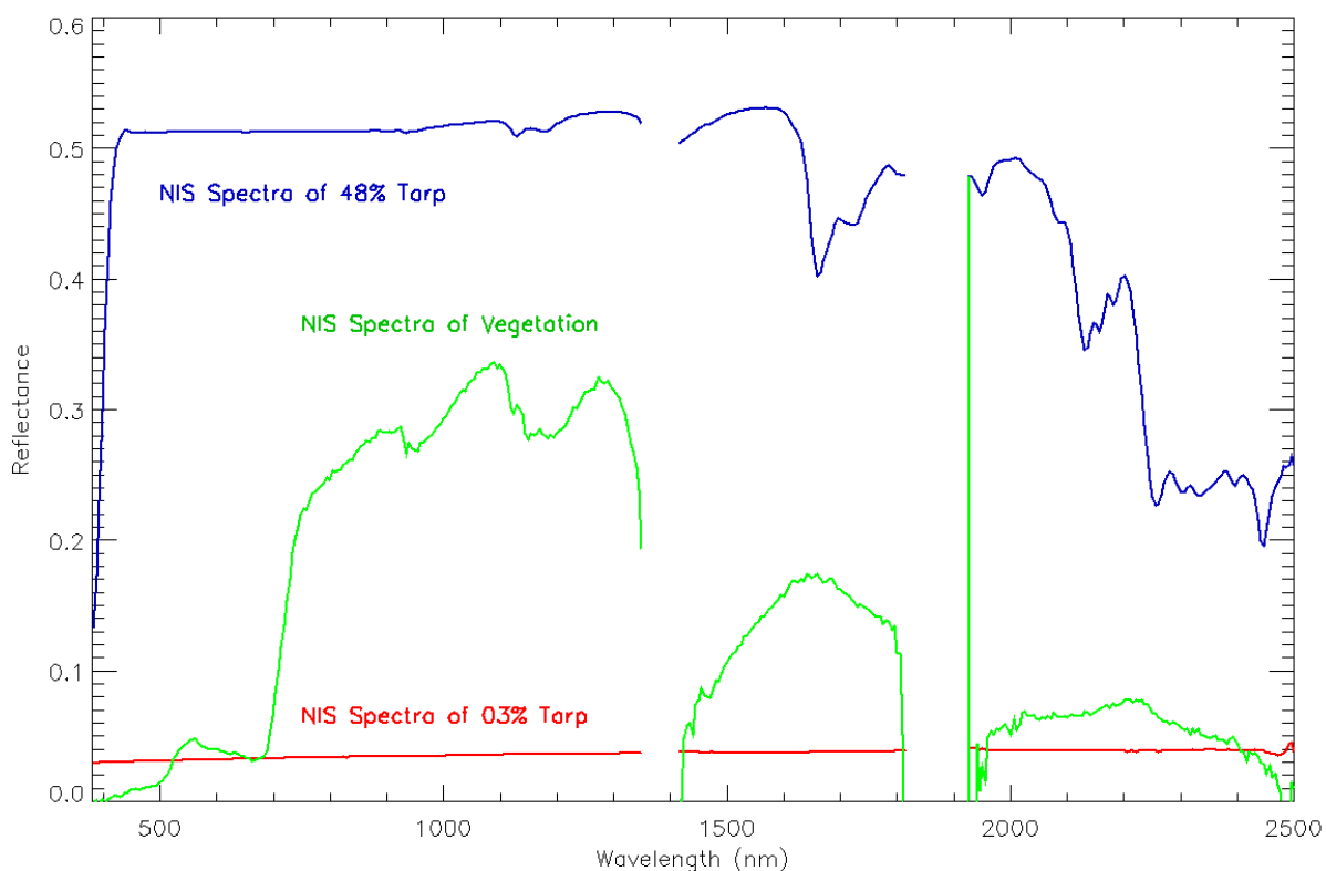
Figure 44: Adjusted reflectance of calibration tarps (03% tarp in red and the 48% tarp in blue) and a vegetation pixel (green) measured by the airborne NEON Imaging Spectrometer
