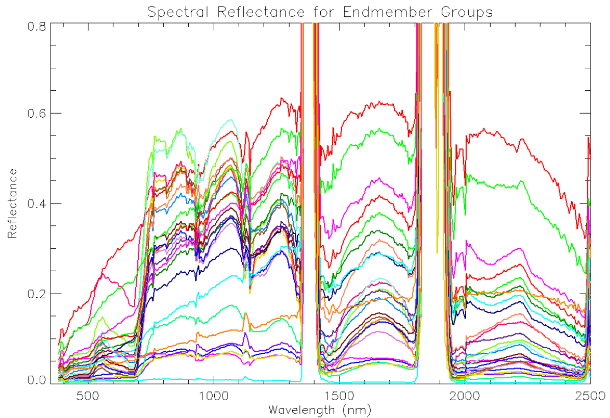
Figure 41: Delivered reflectance versus wavelength for endmembers pixels. Atmospheric artifacts and other noise can be seen in the data
