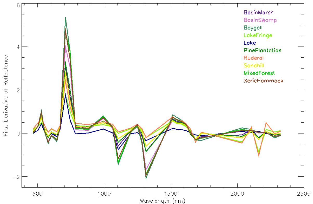
Figure 49: The mean of the first derivative of reflectance of the classification training data for each of the 10 FNAI vegetation communities versus the 32 selected wavelengths
