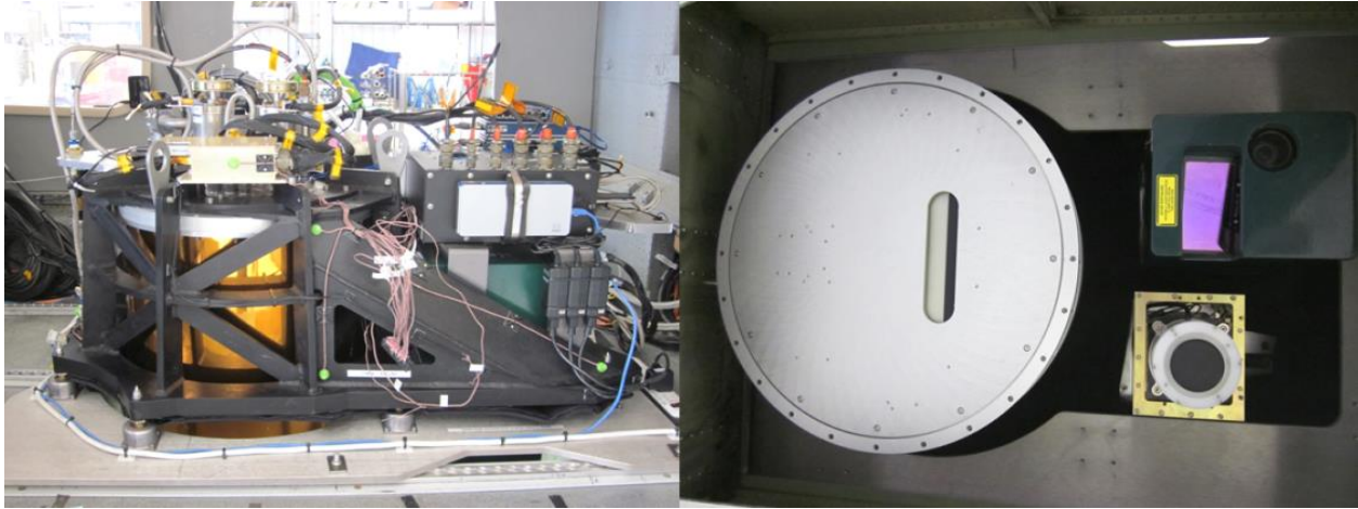
Figure 10: The instruments are mounted in a common rigid frame to improve data co-registration. A side view shown on the left and the view of the instruments from underneath the plane is shown on the right
