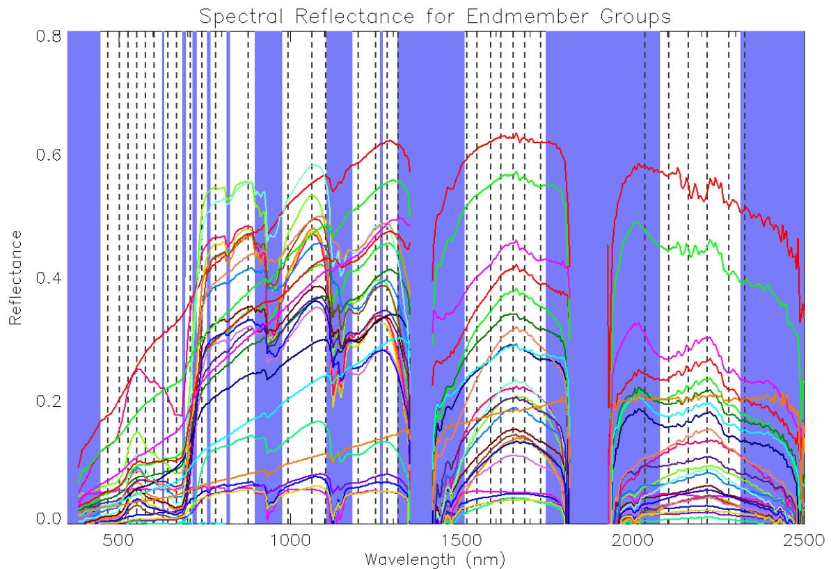
Figure 46: Selection of 32 wavelengths for use in feature calculation, show as the vertical dashed lines on top of the endmember spectra. The blue regions are wavelengths with higher atmospheric absorption
