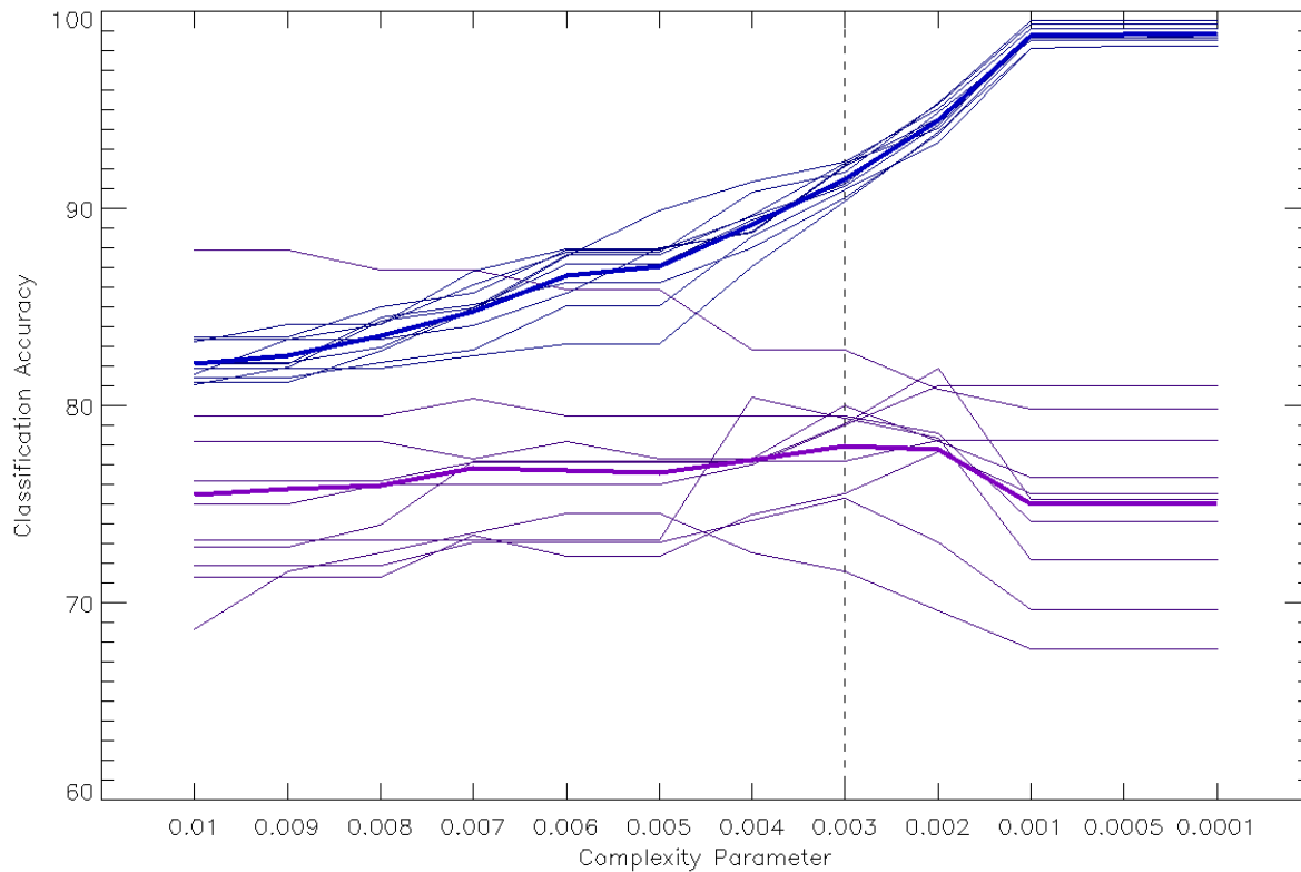
Figure 76: K-folds cross validation to determine the optimal value of the complexity parameter for the integrated hyperspectral and lidar decision tree
