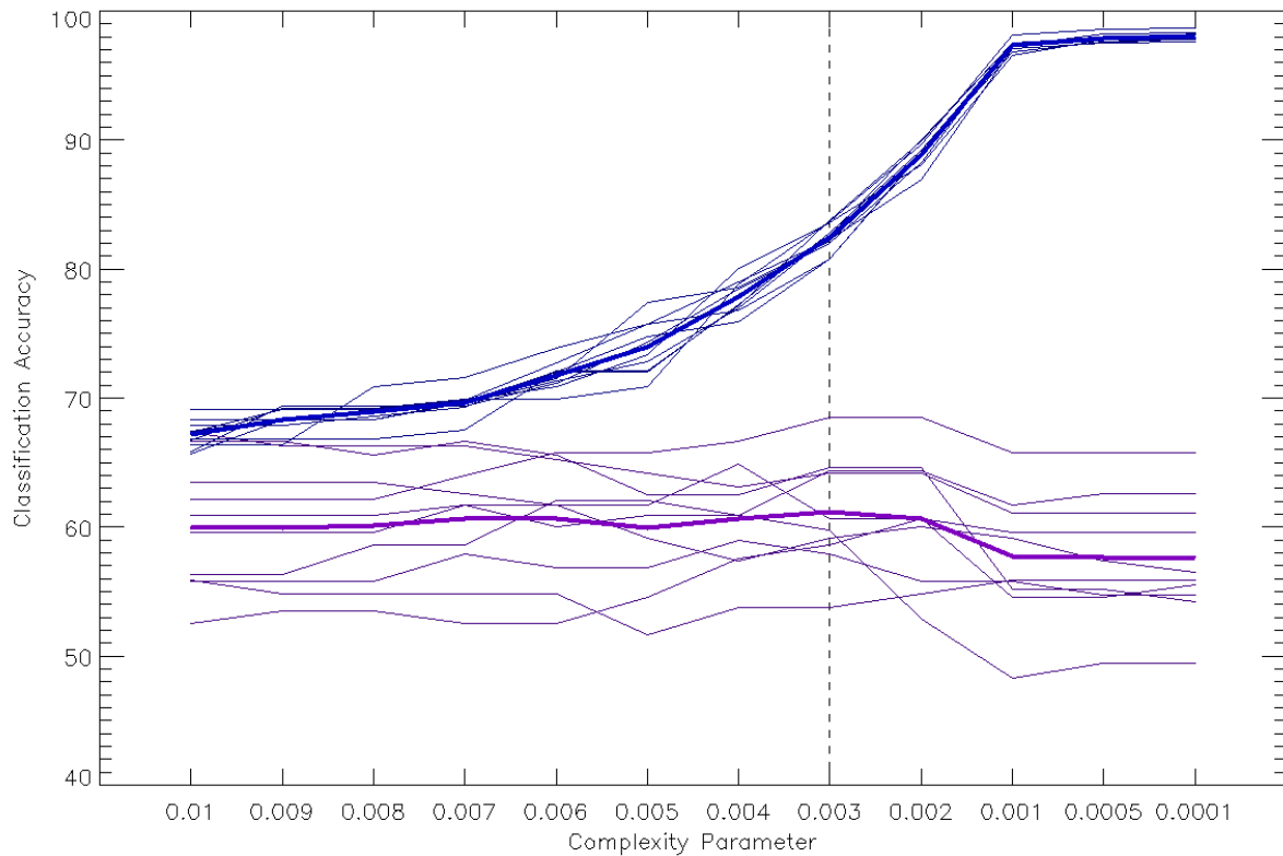
Figure 67: K-folds cross validation to determine the optimal value of the complexity parameter for the lidar decision tree
