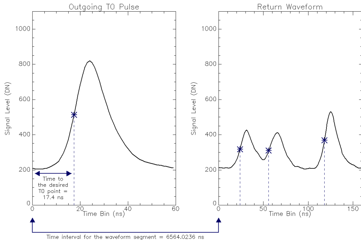
Figure 31: Discrete lidar ranging example using a simple 50% leading edge target detection algorithm
