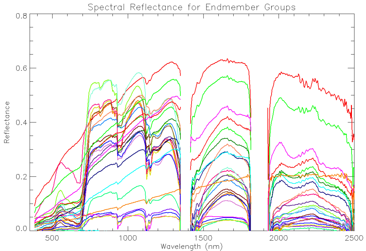
Figure 45: Reflectance versus wavelength for endmembers pixels, adjusted using scale factors generated by using ground calibration tarps
