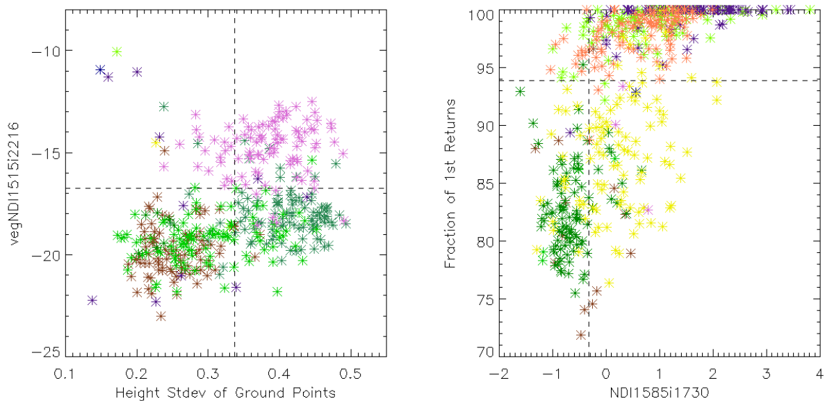
Figure 78: Scatter plots showing how a few of the decision tree splits separate the data. The left side is the normalized difference index for vegetation pixels using the reflectance at wavelengths of 1515 nm and 2216 nm versus the standard deviation of height of the ground points. The right side is the fraction of first returns versus the normalized difference index using the reflectance at wavelengths of 1585 nm and 1730 nm
