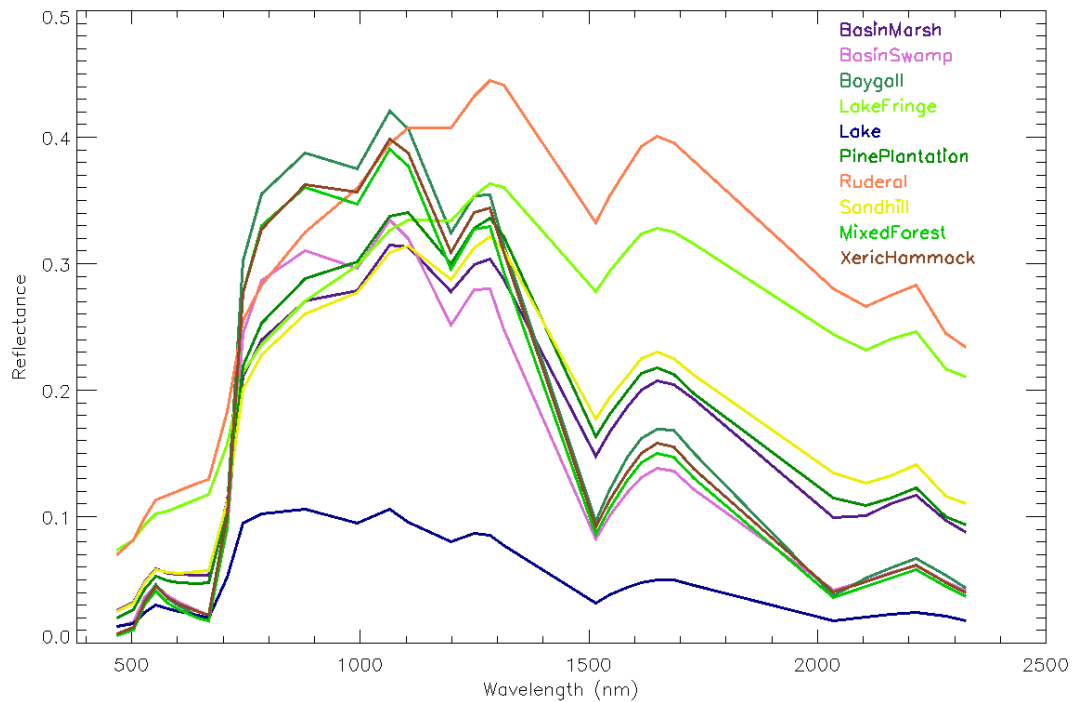
Figure 47: The mean reflectance of the classification training data for each of the 10 FNAI vegetation communities versus the 32 selected wavelengths
