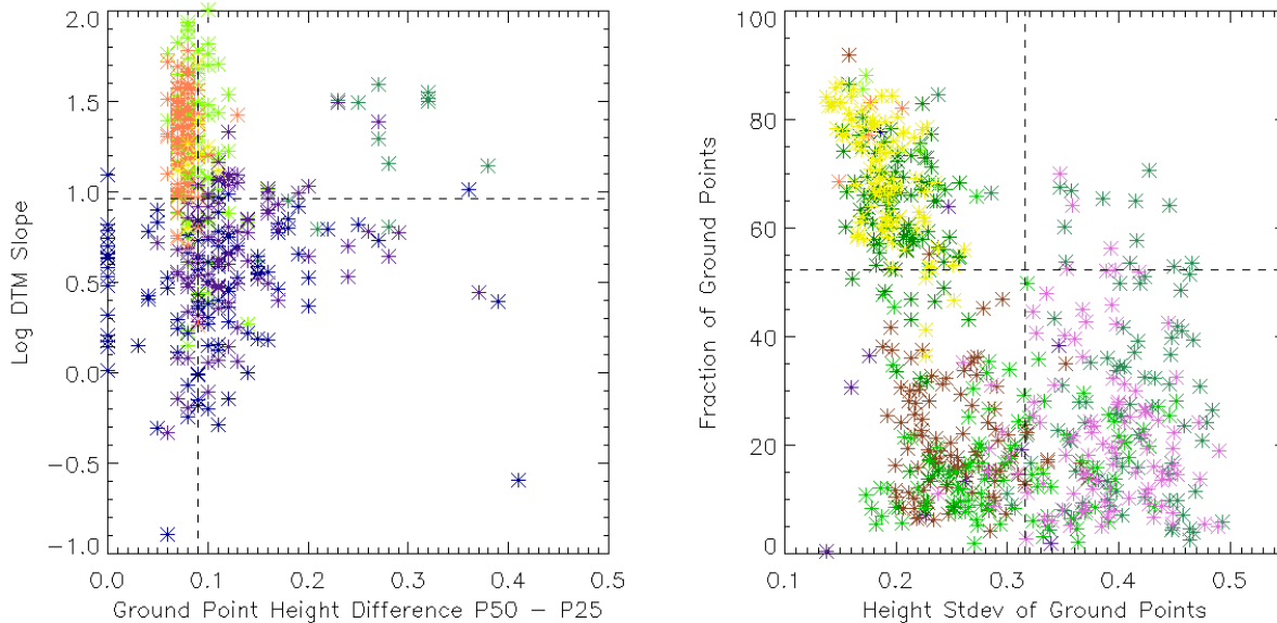
Figure 70: Scatter plots showing how a few of the decision tree splits separate the data. The left side is the log of the coarse resolution bare-Earth slope versus the height difference of the 50 th minus 25 th percentile height of ground points. The right side is fraction of ground points versus the standard deviation of height of the ground points
