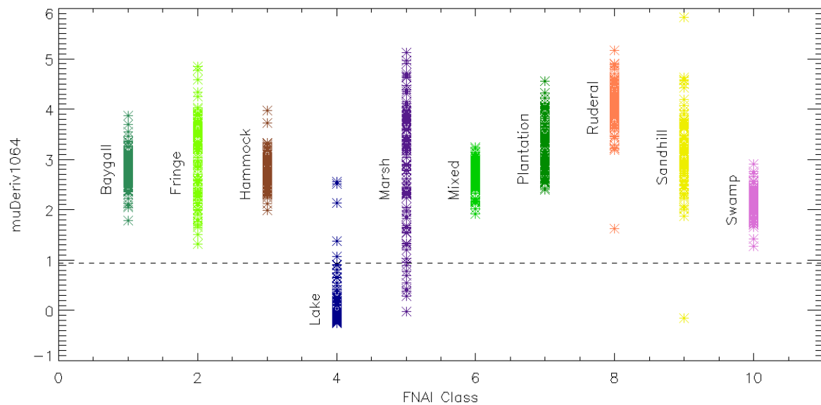
Figure 54: Mean of the first derivative of reflectance at 1064nm as the first split of the decision tree, separating Lake areas from the other vegetation communities
