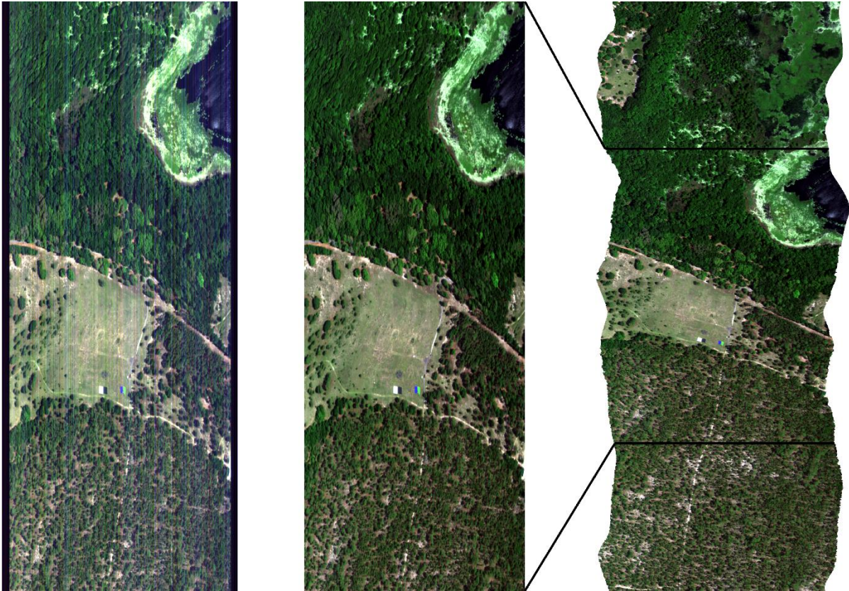
Figure 28: Radiometric correction and ortho-rectification of a portion of a single flight line of imaging spectrometer data. The left image is the raw data in the native 2D sensor rectangular format collected by the spectrometer where vertical radiometric streaks are visible. The center image has been converted to radiance, removing the streaks, but showing wavy lines due to aircraft turbulence and is oversampled by a factor of two in the along-track direction. The flight line is ortho-rectified onto a fixed 1 m output grid with a WGS84 UTM projection using nearest neighbor resampling as shown on the right
