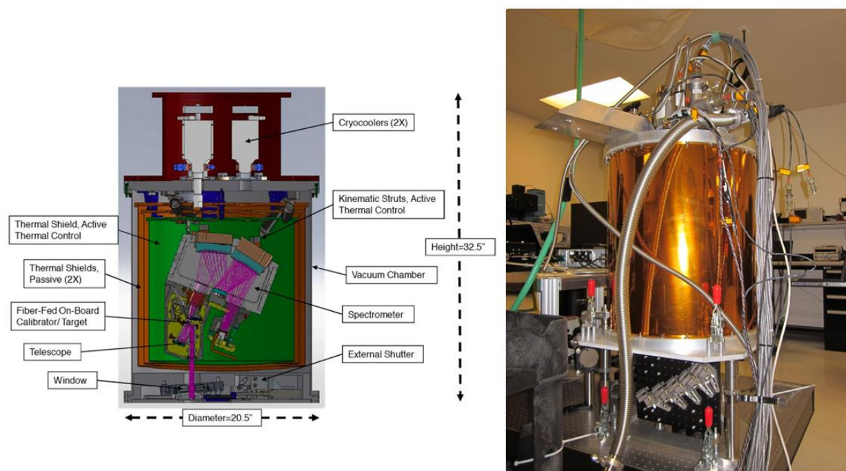
Figure 6: Schematic of the NEON Imaging Spectrometer on the left (figure courtesy of NASA JPL) and a picture of the instrument in the lab on a test fixture on the right
