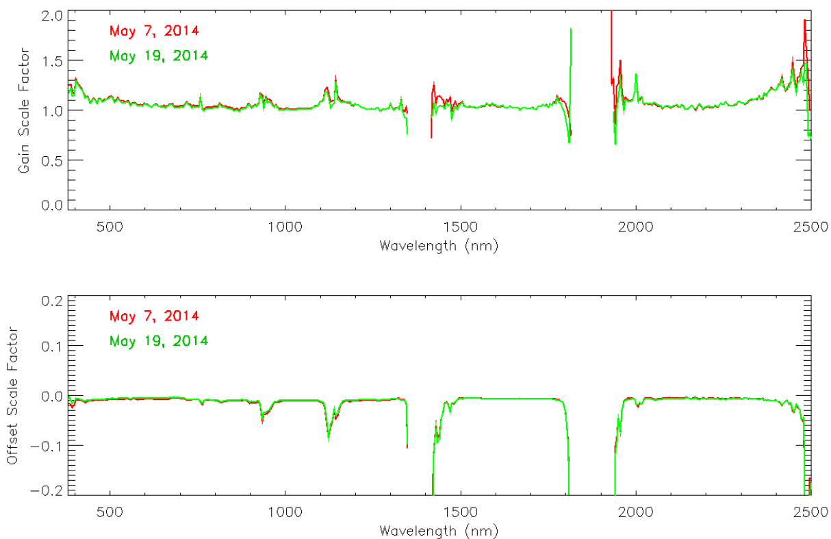
Figure 43: Gain and offset coefficients used in the empirical line adjustment to improve the quality of the NEON Imaging Spectrometer reflectance products collected on May 7 and May 19, 2014 at Ordway-Swisher Biological Station
