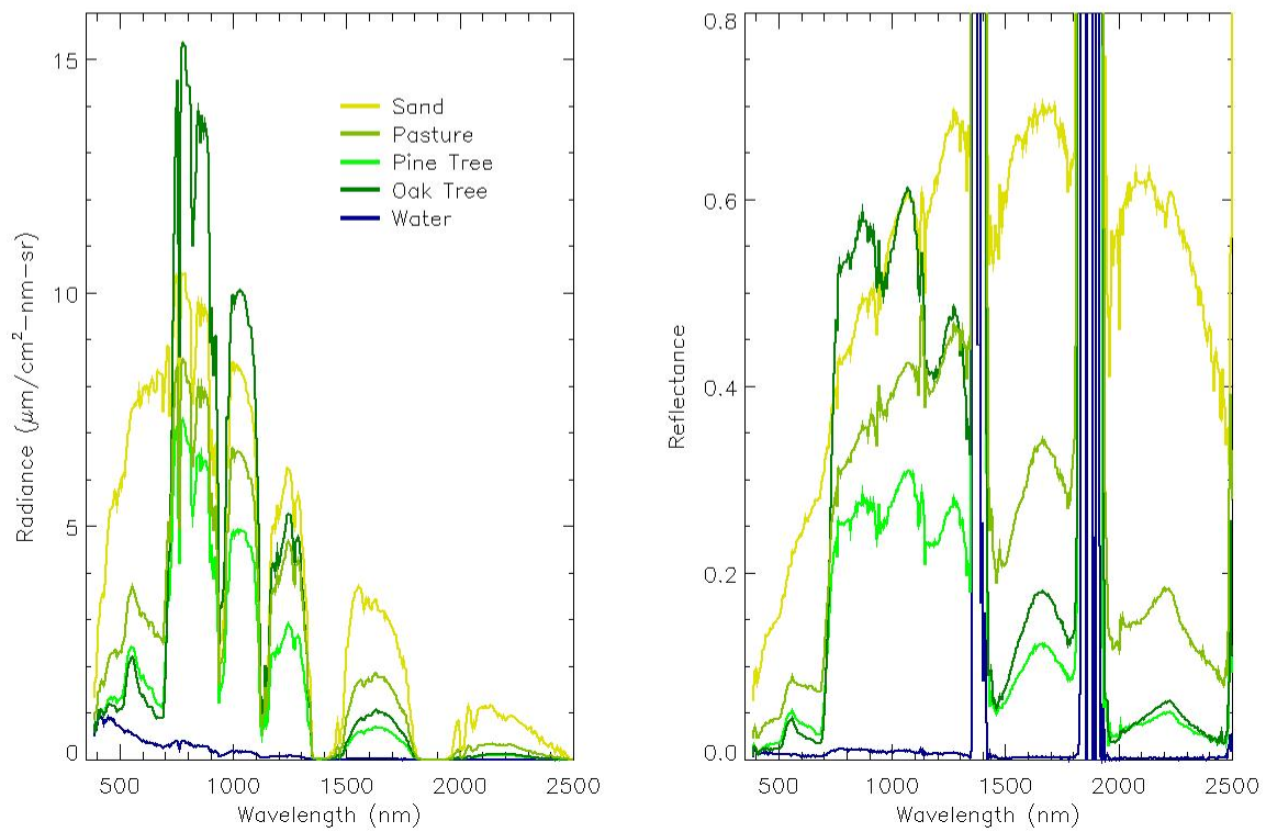
Figure 29: At-sensor radiance (bottom left) and directional surface reflectance (bottom right) curves for several natural targets whose spatial locations are shown in the top of the figure
