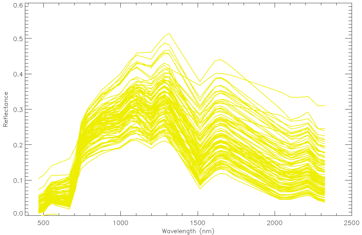
Figure 48: Plot level mean reflectance versus the 32 selected wavelengths for all 100 of the Sandhill training locations
